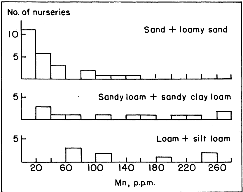
Fig. 23. Soil manganese for 45 southern forest nurseries.
