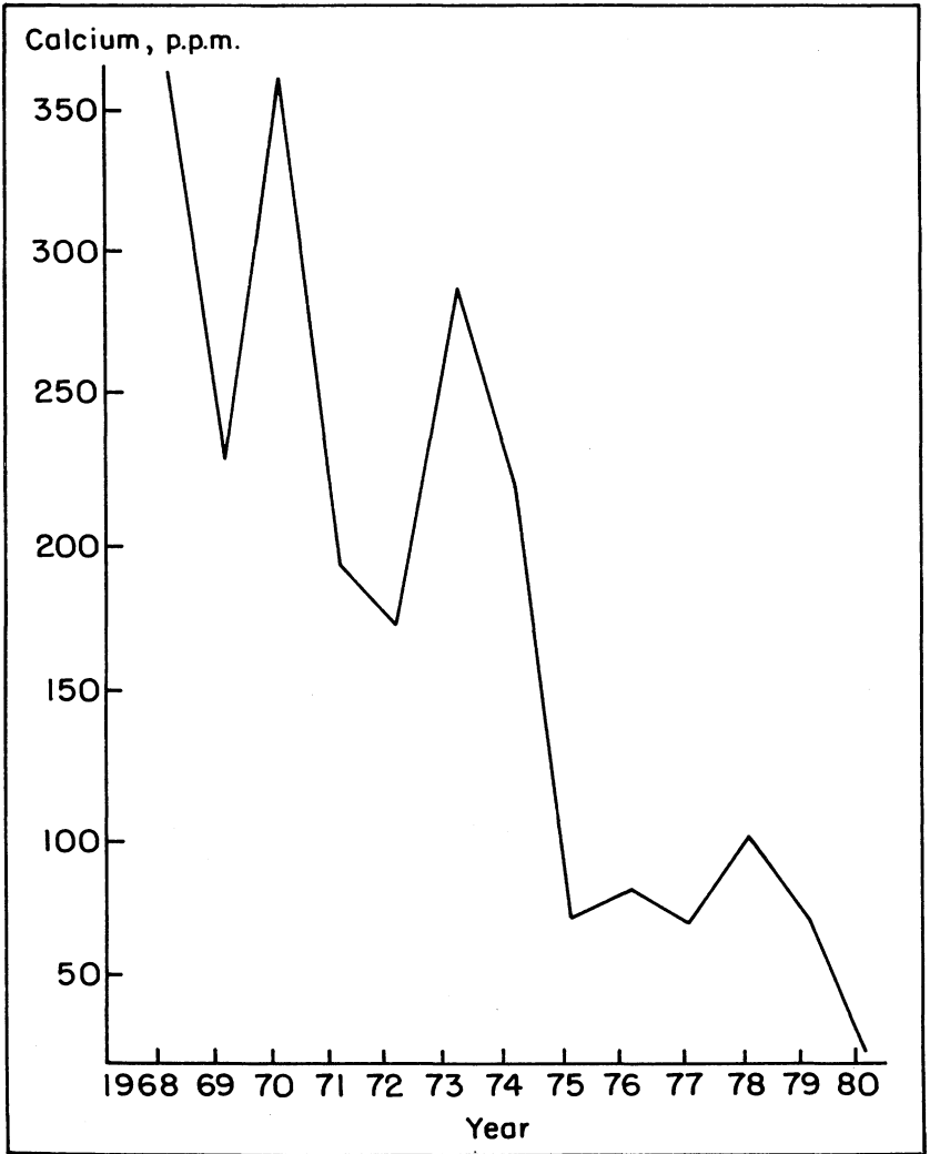
Fig. 4. History of soil calcium for one compartment in a southern forest tree nursery.
