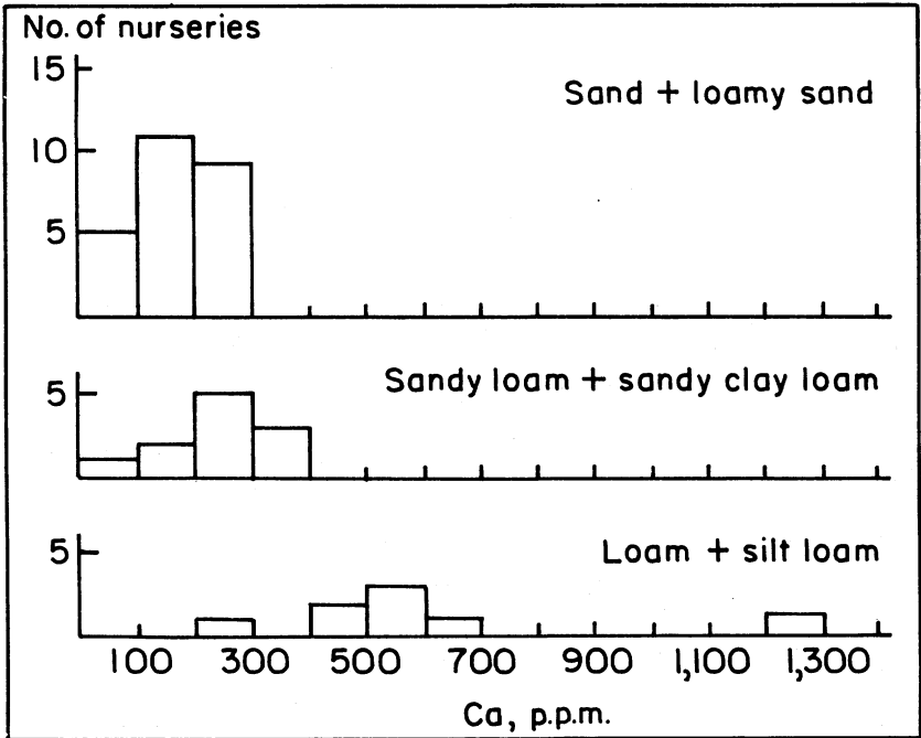
Fig. 16. Soil calcium for 45 southern forest nurseries.
