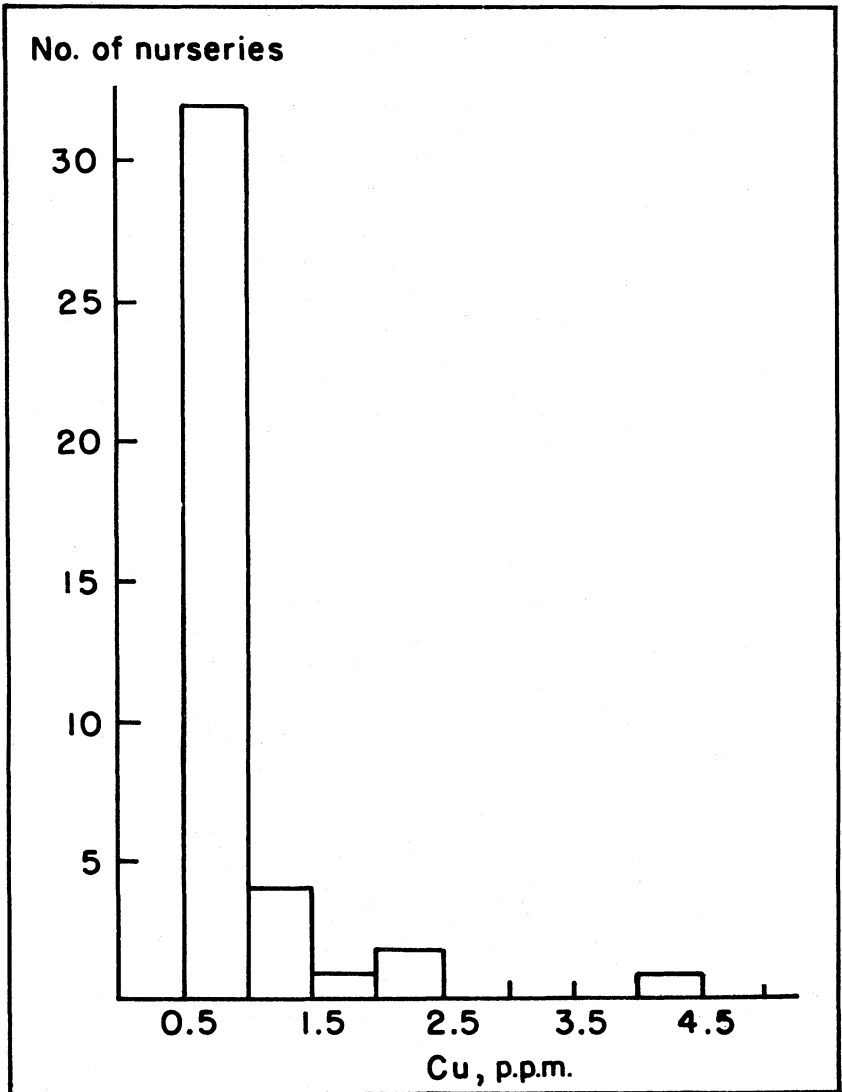
Fig. 25. Soil copper for 45 southern forest nurseries.
