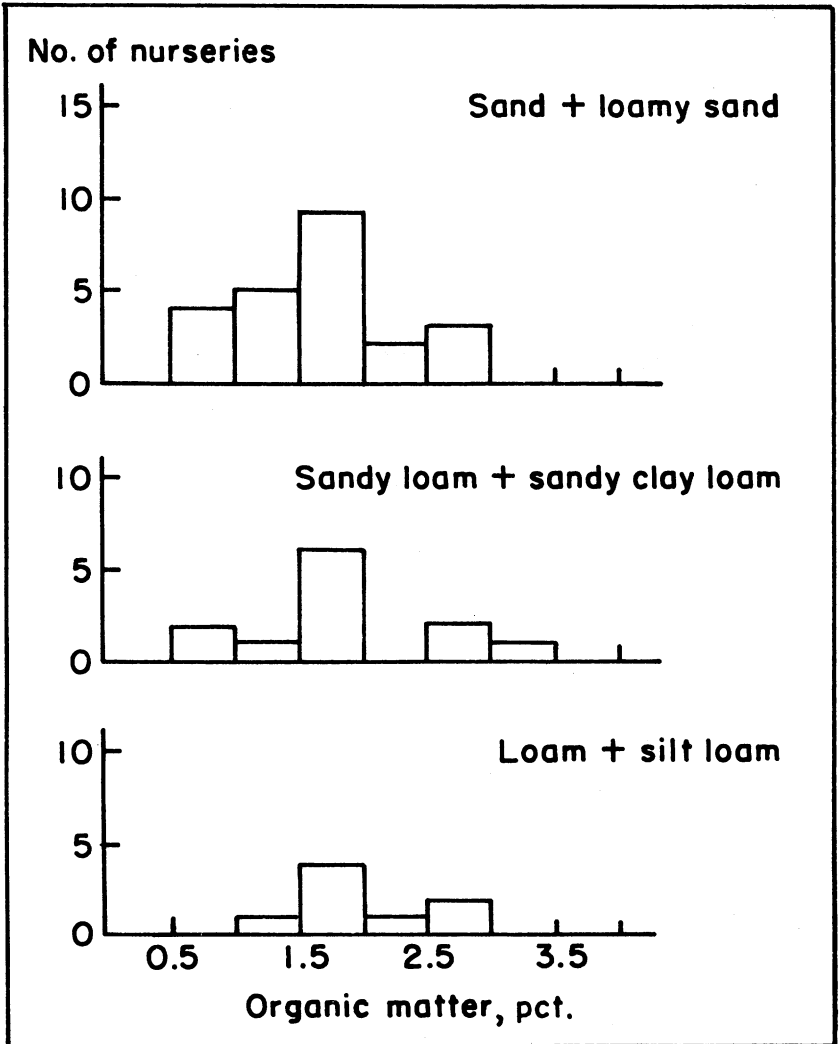
Fig. 10. Organic matter content for 45 southern forest nurseries.
