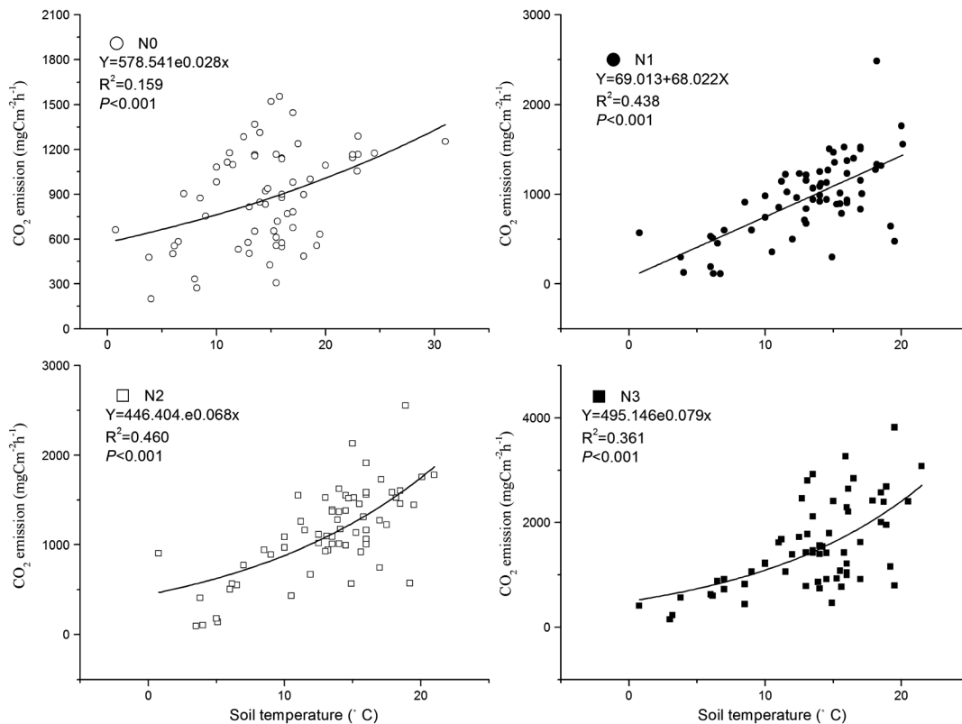
Figure 5. The relationship between CO 2 flux rate and soil temperature at 5 cm depth. N0, 0 kg N ha -1 yr -1 ; N1, 60 kg N ha -1 yr -1 ; N2, 120 kg N ha -1 yr -1 ; N3, 240 kg N ha -1 yr -1 .
