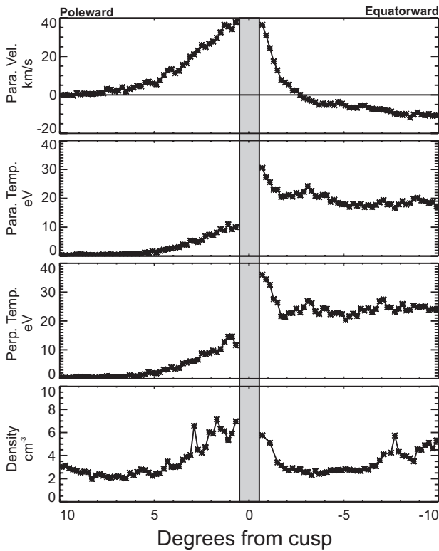
Figure 8. Plots of the average plasma moments as calculated from the fitted ionosphere. These moments are plotted as a function of distance from the magnetosheath precipitation boundary as measured by TIDE. Format of this plot is the same as that in Figures 4 and 5. The gray bar through the panels \pm 0.5^\circ the magnetosheath precipitation boundary indicates the region of poor confidence in the ionospheric fitting procedure.
