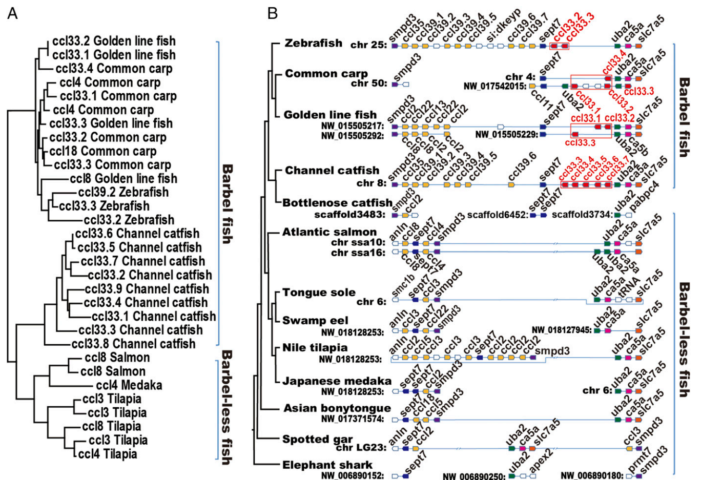
Fig. 2. Chemokine ccl33 genes were identified to be specific in barbeled fish. (A) Phylogenetic clade containing chemokine ccl33 genes was only present in barbeled fish. (B) Conserved syntenic region that included the ccl33 (in red box) genes was specific in barbeled fish.
