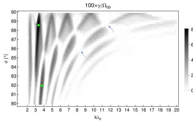
Figure 7. Linear theory growth rate ( \gamma ) as a function of the wave number ( k ) and the wave normal angle ( \psi ) for Case II. The filled green circle denotes the maximum growth rate of \gamma = 0.081\Omega_{cp} located at \psi = 88.6^\circ and k\lambda_p = 3.35 . The filled green square denotes the second local maximum growth rate of \gamma = 0.059\Omega_{cp} located at \psi = 82^\circ and k\lambda_p = 3.75 . Two arrows indicate the growth rate gaps for the \omega \sim 7\Omega_{cp} mode.
