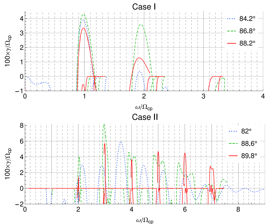
Figure 13. Linear theory growth rates as a function of the real frequency for (top) Case I and (bottom) Case II. The three curves in each panel correspond to growth rates for three different wave normal angles as denoted by the legends.
