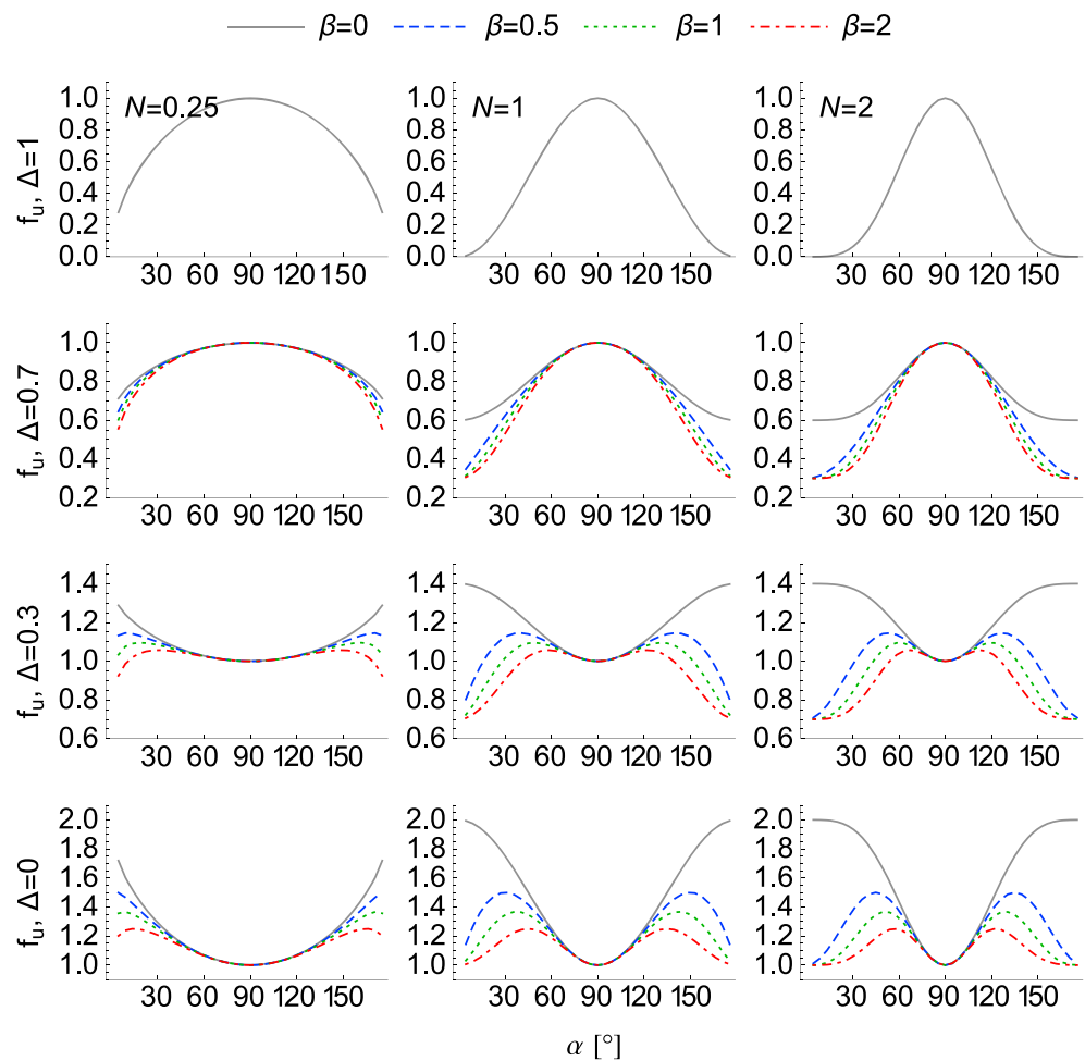
Figure 3. Pitch angle dependence of the base distribution function of equation (1) used to fit the observed ion fluxes. Four \Delta values (1, 0.7, 0.3, and 0), three N values (0.25, 1, and 2), and four \beta values (0, 0.5, 1, and 2) are chosen for illustration.
