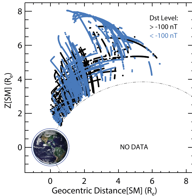
Figure 14. Geocentric distance and Z component of all S/C locations in solar magnetic (SM) coordinates when a LAE is observed. Blue dots indicate locations during moderate or stronger storm activity. Locations from \sim 2-3R_e or further out observe source emissions from the opposite hemisphere. Higher latitudes at the S/C location reflect a lower latitude on the opposite hemisphere.
