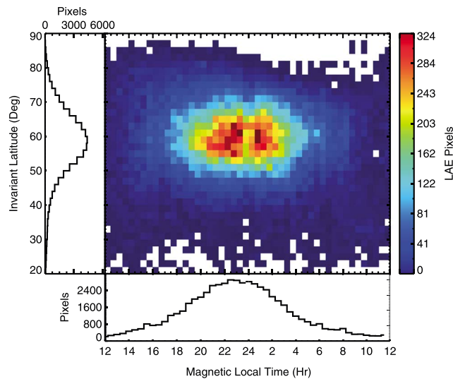
Figure 12. Magnetic local time and invariant latitude correlation of LAE pixels. The MLT is roughly centered just before midnight, and the IL peaks slightly below 60° latitude.
