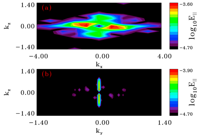
Figure 11. Spectrum of the elongated E_{\parallel} structure at the leading wave front for Case 3 in the (a) k_x - k_z space at y = 32 and (b) k_y - k_z space at x = 13 .
