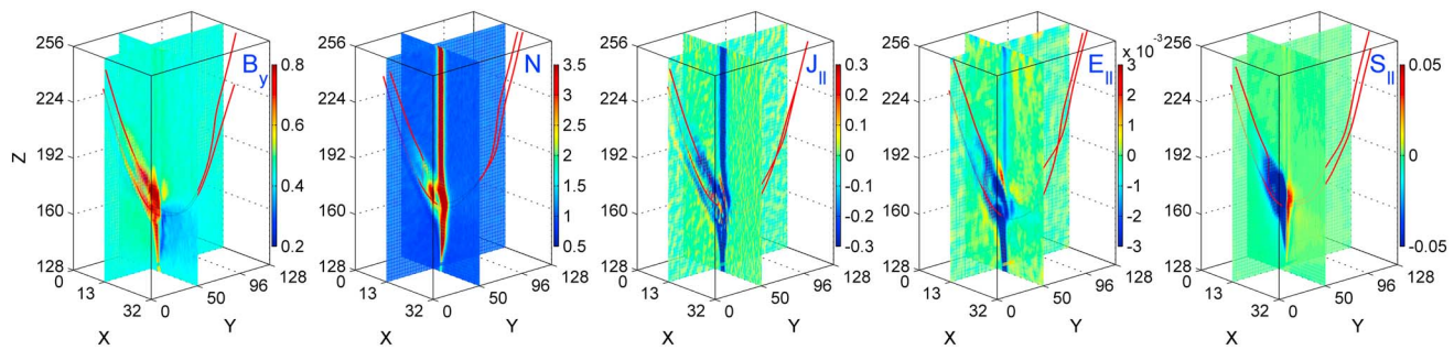
Figure 14. Contours for Case 4 in 3-D of B_y , N , J_{\parallel} , E_{\parallel} , and S_{\parallel} , with several magnetic field lines, at t = 150 . The two slices are at x = 13 and y = 50 .
