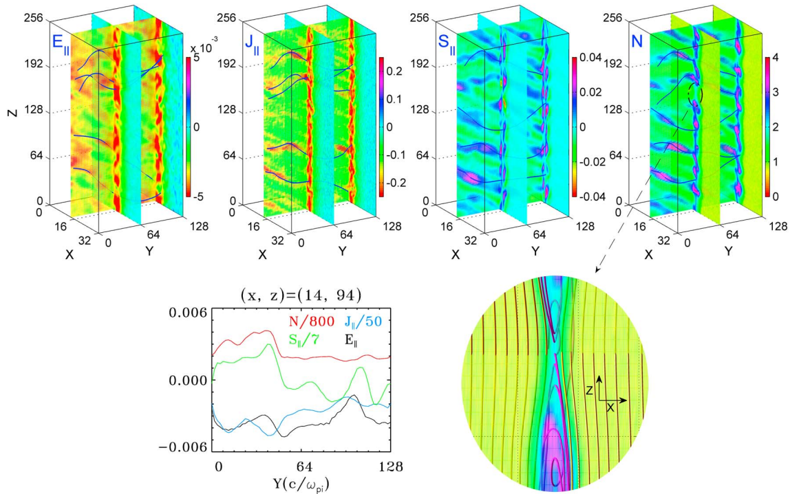
Figure 1. (top row) Overall views of parallel electric field E_{\parallel} , parallel current J_{\parallel} , parallel Poynting flux S_{\parallel} , and ion density N , with some typical magnetic field lines in 3-D view, and (bottom row) spatial cuts of the quantities along y as well as a zoomed-in plot of the density (with field lines) obtained from the simulation of Case 1 at t = 300 . The contours are shown for three planes of x = 14 , y = 64 , and y = 128 .
