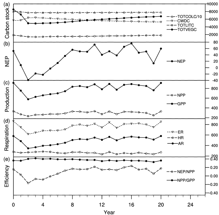
Figure 14. Simulated postfire temporal evolution of carbon budget and ecosystem productivity based on the idealized burning experiment. (a) Total column carbon ( \text{g C}/\text{m}^2 ), coarse woody debris carbon ( \text{g C}/\text{m}^2 ), total litter carbon ( \text{g C}/\text{m}^2 ), and total vegetation carbon ( \text{g C}/\text{m}^2 ); (b) net ecosystem production ( \text{g C}\cdot\text{m}^{-2}\cdot\text{year}^{-1} ); (c) net primary production ( \text{g C}\cdot\text{m}^{-2}\cdot\text{year}^{-1} ) and gross primary production ( \text{g C}\cdot\text{m}^{-2}\cdot\text{year}^{-1} ); (d) total ecosystem respiration ( \text{g C}\cdot\text{m}^{-2}\cdot\text{year}^{-1} ), heterotrophic respiration ( \text{g C}\cdot\text{m}^{-2}\cdot\text{year}^{-1} ), and autotrophic respiration ( \text{g C}\cdot\text{m}^{-2}\cdot\text{year}^{-1} ); (e) ecosystem carbon storage efficiency (unitless) and plant production efficiency (unitless). The time of fire disturbance is at year 0.
